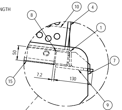
DETAIL A (1 : 5)
